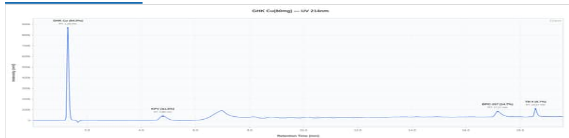
KLOW 80mg 80mg - Purple lids/silver crimps: UV Chromatogram
